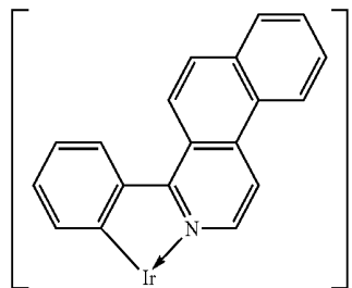
Compound A1
