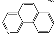
Benzo[h]isoquinoline
