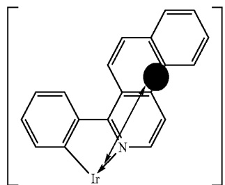
Compound A1
