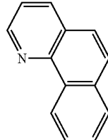
Benzo[h]quinoline
